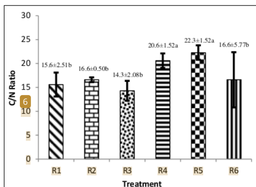
Figure 4. Characteristics of C/N ratio of compost using a combination of CF with WH in different ratios and WRF ( Ganoderma sp ) as decomposer; (R 1 )(CF:WH)(25%:75%)+WRF; (R 2 )(CF:WH)(50%:50%)+WRF; (R 3 )(CF:WH)(75%:25%)+WRF; (R 4 )(CF:WH)(25%:75%) without WRF; (R 5 )(CF:WH)(50%:50%) without WRF; and (R 6 )(CF:WH)(75%:25%)+without WRF; a,b Different scripts show significant differences ( p < 0.05 ); Fermentation time=30 days; CF=cattle feces; WH=water hyacinth ( Eichhornia crassipes ); WRF= white rot fungi ( Ganoderma sp )
